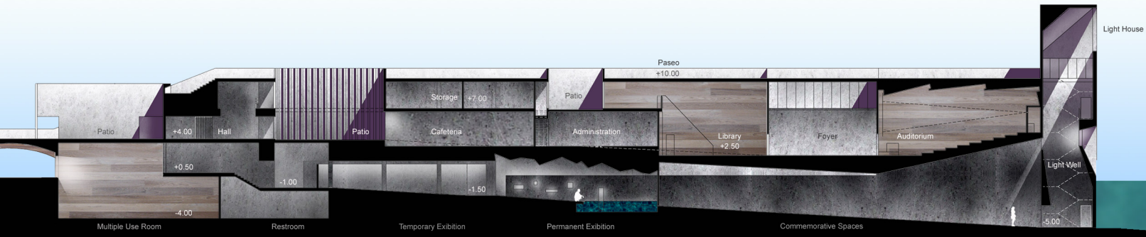
Longitudinal Section Total covered surface: 2091mq
